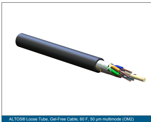
ALTOS® Loose Tube, Gel-Free Cable, 60 F, 50 µm multimode (OM2)
