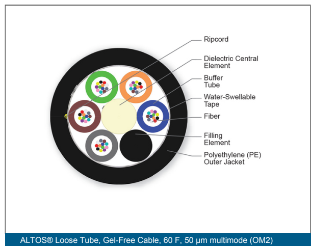
ALTOS® Loose Tube, Gel-Free Cable, 60 F, 50 µm multimode (OM2)
